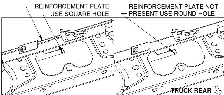
3500 TRUCK WITH REINFORCEMENT PLATES 3500 TRUCK WITHOUT REINFORCEMENT PLATES
